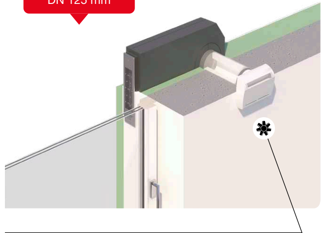
Install. example DN 125 mm
